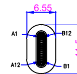
VIEW B
